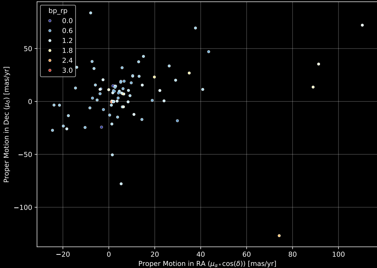
APOGEE DR17 Field: [281-35-O] Proper Motion Diagram (n= 122)
