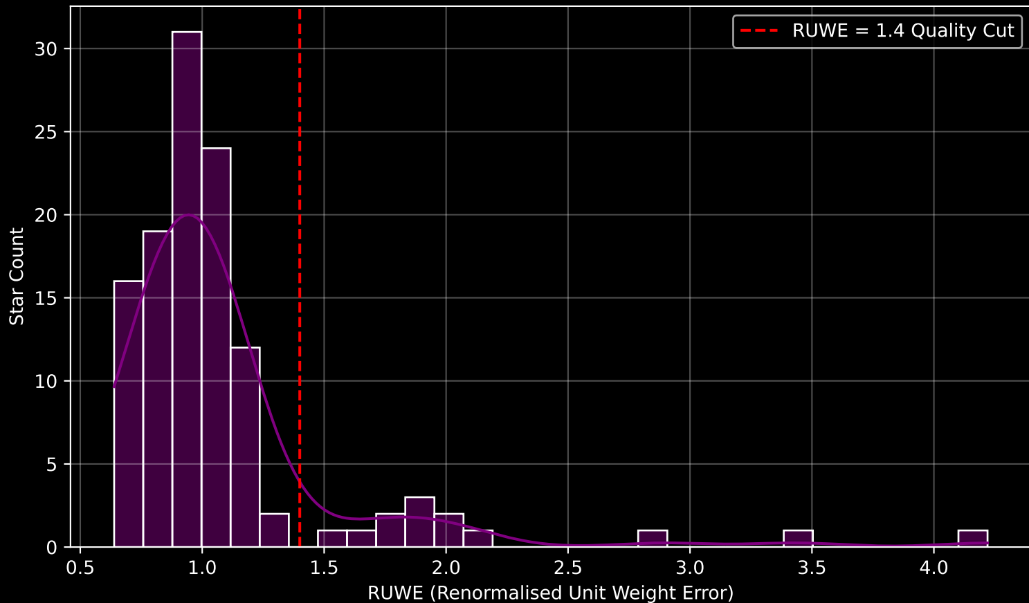
GAPOGEE DR17 Field [281-35-O] RUWE Distribution (n= 117)
