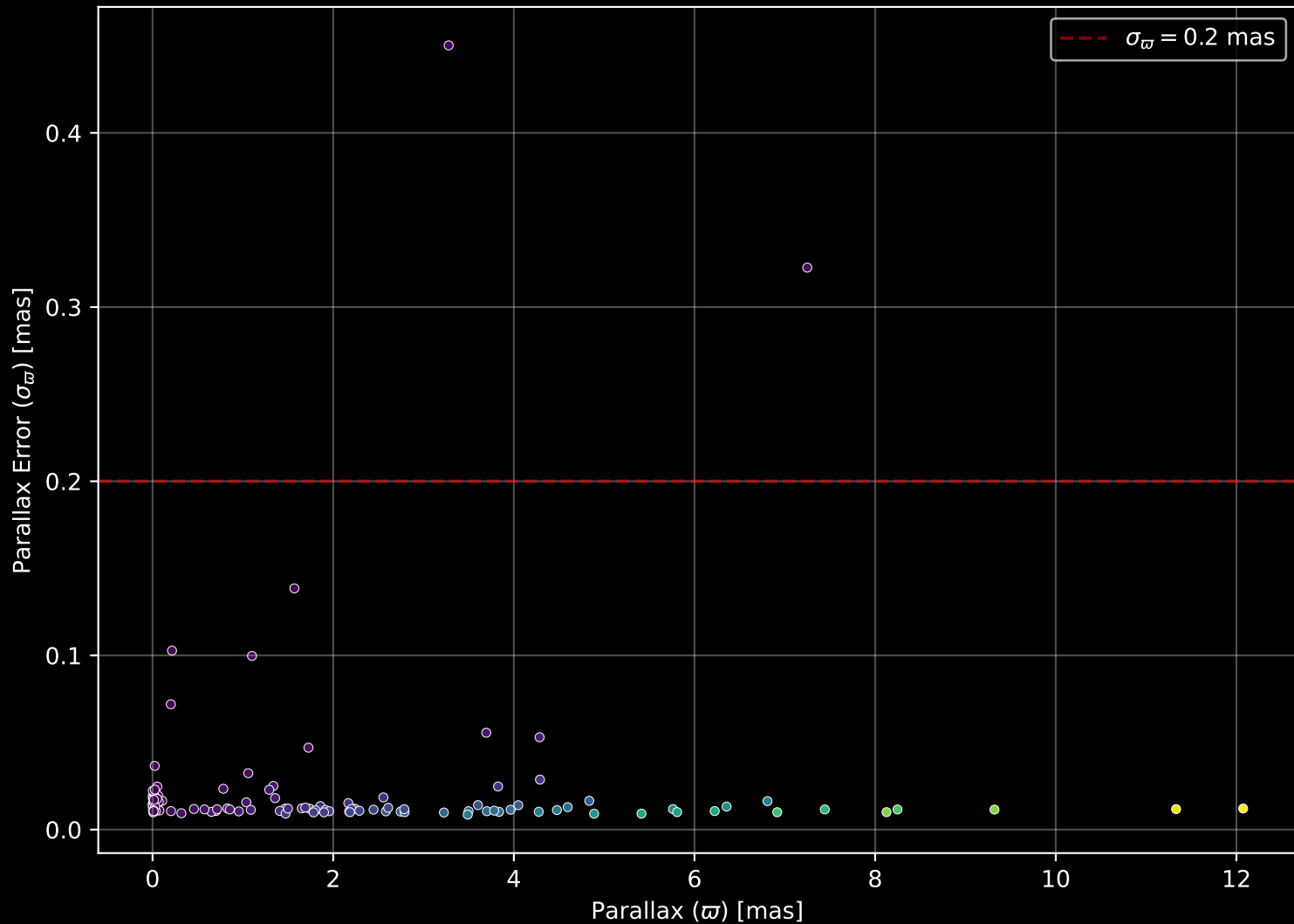
APOGEE DR17 Field: [281-35-O] Parallax Quality (n= 122)
