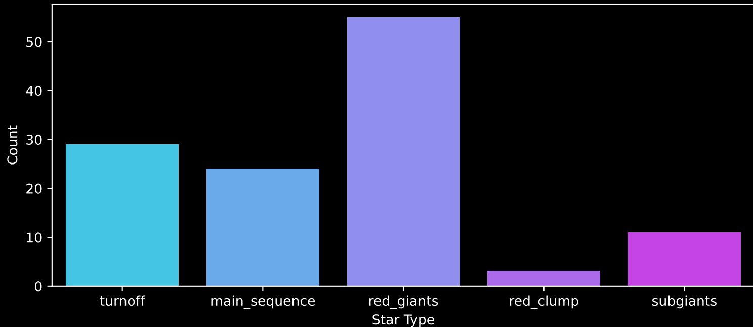
APOGEE DR17 Field: [281-35-O] Count plot of Star Type
