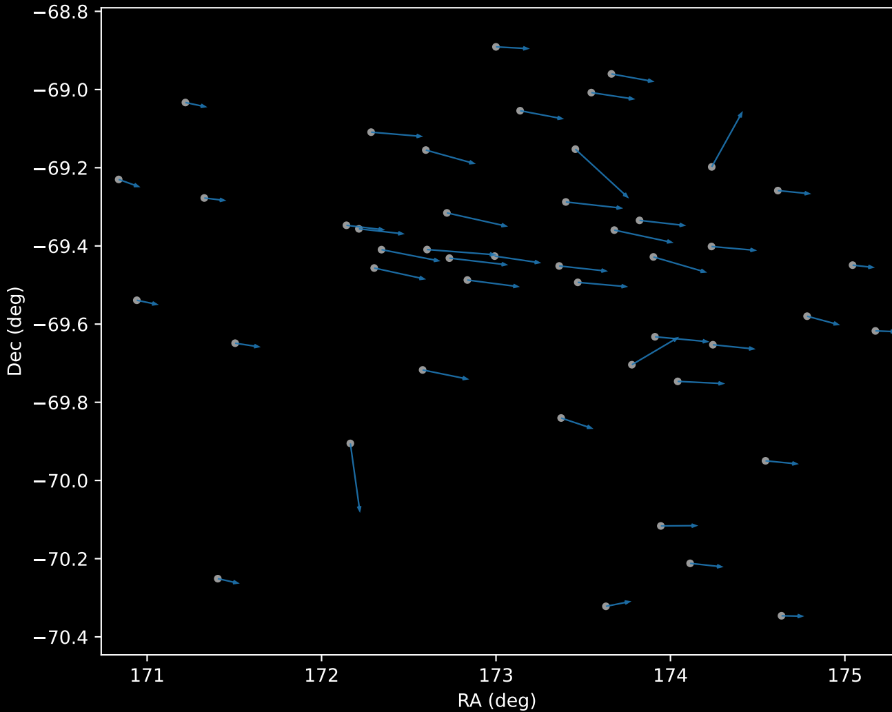
APOGEE DR17 Cluster 0 Proper Motion Vectors (n=46)
